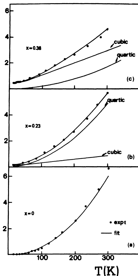
FIG. 3. A_{1g} linewidth behavior as a function of temperature for three different cadmium concentrations. The cubic and quartic anharmonic contributions are found by means of Eq. (2) in the text.
