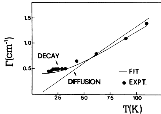
FIG. 4. A_{1g} linewidth for x=0.38 between 20 and 120 K. Solid lines represent the best fitting of the experimental data (points) when decay or diffusion processes are considered.
