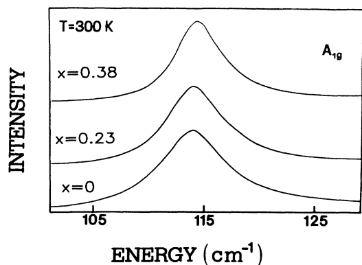
FIG. 1. Room-temperature spectra of the A_{1g} mode in Cd_xHg_{1-x}I_2 ( x = 0, 0.23, \text{ and } 0.38 ).
