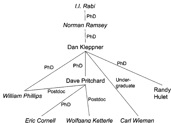
FIG. 10. Family tree of atomic physicists. People with names in italics are Nobel laureates.
