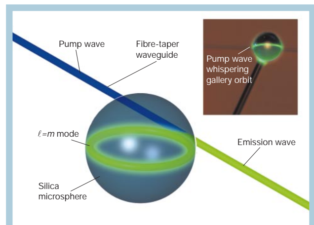
Figure 5 Illustration of a silica microsphere whispering gallery resonator. The green orbit is a l=m mode entrained at the sphere's surface. Also shown is a fibre taper waveguide used for power coupling to and from the resonator. In the figure, a blue pump wave induces a circulating intensity within the sphere that is sufficient to induce laser oscillation (green emission wave). Inset: Photomicrograph showing a doped microsphere (the glass sphere contains a rare earth). The green emission in this case traces the pump wave whispering gallery orbit. The inset micrograph was provided by M. Cai.
