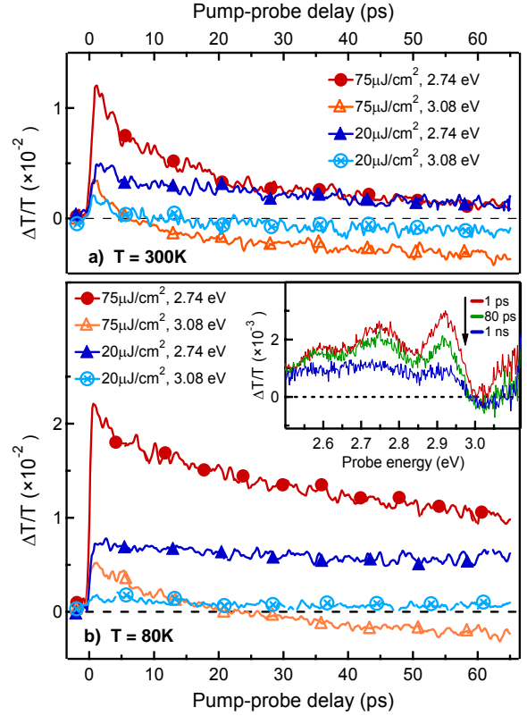
Figure 3. \Delta T/T time traces taken for different pump fluences and probe photon energies at T = 300 (a) and 80 K (b); pump photon energy: h\nu_p = 3.54 eV. Inset of panel (b): Near-gap \Delta T/T spectra measured for \Phi_{ex} \sim 10 \mu\text{J}/\text{cm}^2 .
