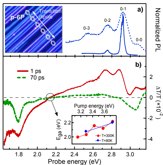
Figure 1. Panel a): cw-spontaneous emission (dotted curve) and amplified spontaneous emission (continuous curve) spectrum at T = 300 K. Inset: Fluorescence image of a 140 \times 110 \mu\text{m}^2 region of an epitaxially grown p -6P thin film featuring sparse needles. Panel b): Differential transmission ( \Delta T/T ) spectra taken at T = 300 K for various pump-probe delays; excitation energy fluence: \Phi_{\text{ex}} = 90 \mu\text{J}/\text{cm}^2 per pulse; pump photon energy: h\nu_p = 3.44 eV. Polarization of the probe beam is parallel to the molecular axis. Inset: gain-to-absorption cross-over energy (isosbestic point) measured at zero delay versus pump photon energy.
